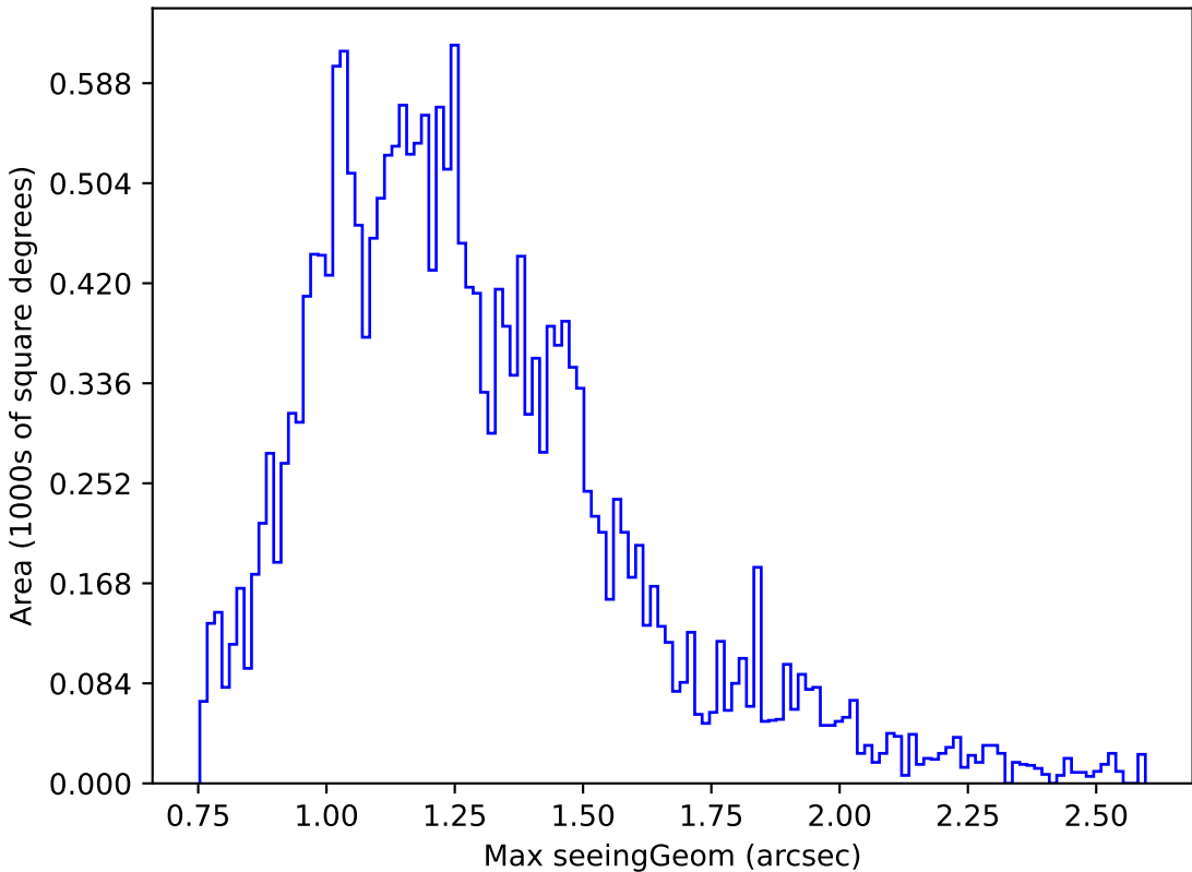
weather_cloudso6v3.4_10yrs Yr 1 u band: Max seeingGeom
