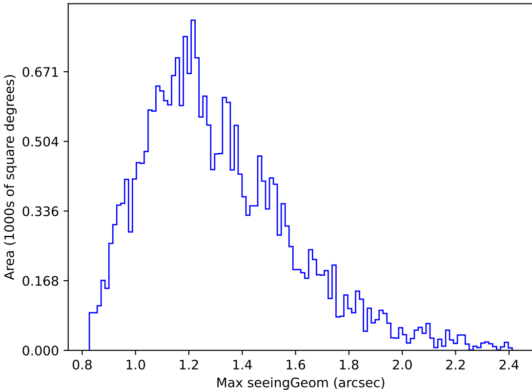
weather_cloudso6v3.4_10yrs Yr 1 i band: Max seeingGeom
