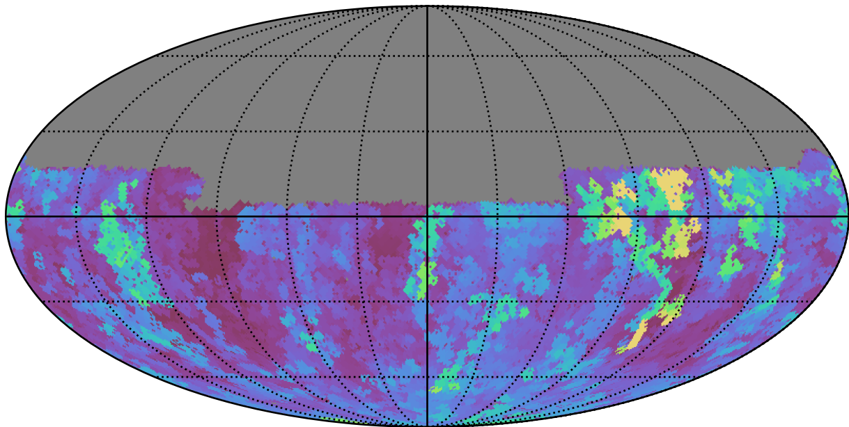
weather_cloudso6v3.4_10yrs Yr 1 u band: Max seeingEff
