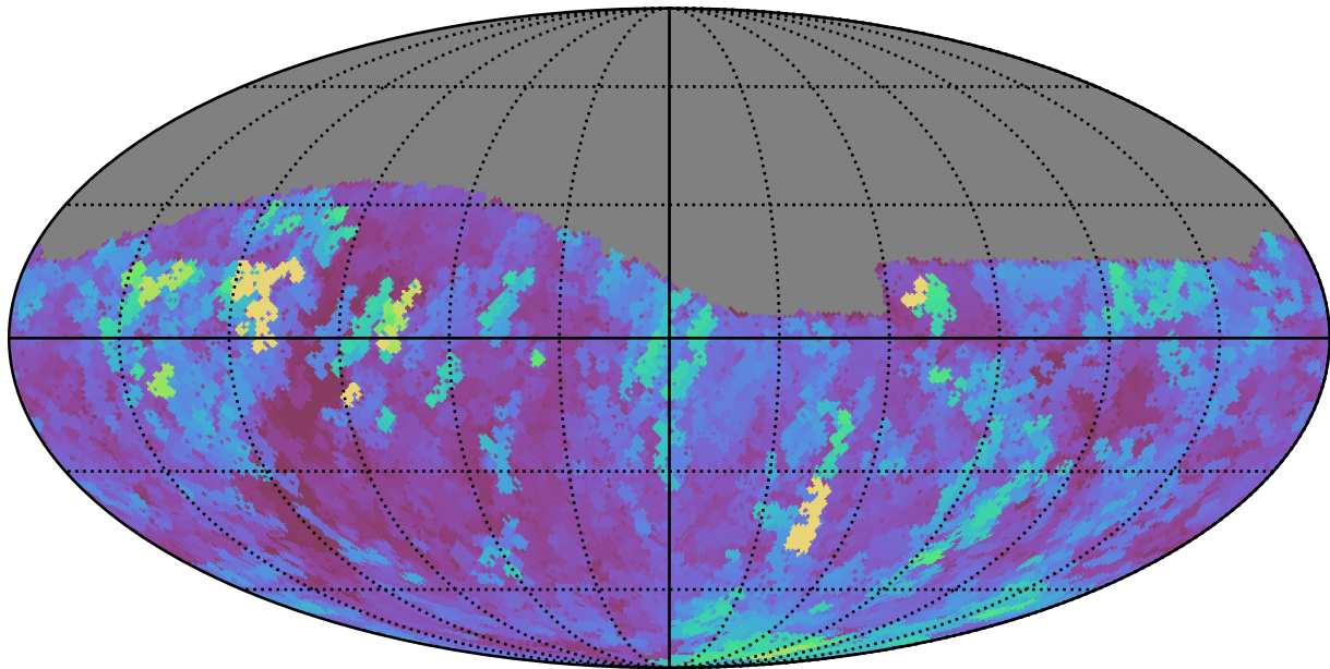
weather_cloudso6v3.4_10yrs Yr 1 r band: Max seeingEff
