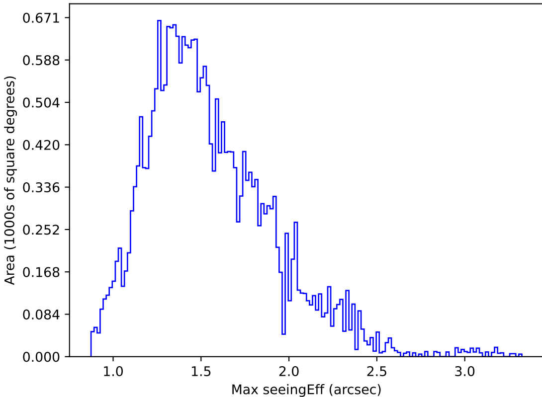
weather_cloudso6v3.4_10yrs Yr 1 r band: Max seeingEff
