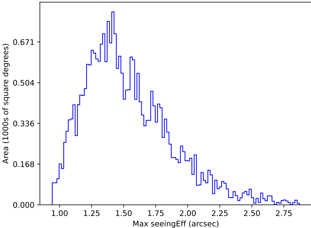
weather_cloudso6v3.4_10yrs Yr 1 i band: Max seeingEff
