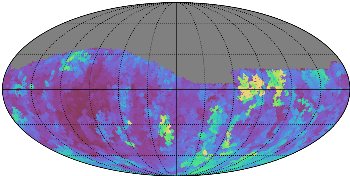
weather_cloudso6v3.4_10yrs Yr 1 g band: Max seeingEff
