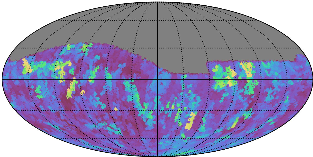
weather_cloudso6v3.4_10yrs Yr 1 all bands: Max seeingEff
