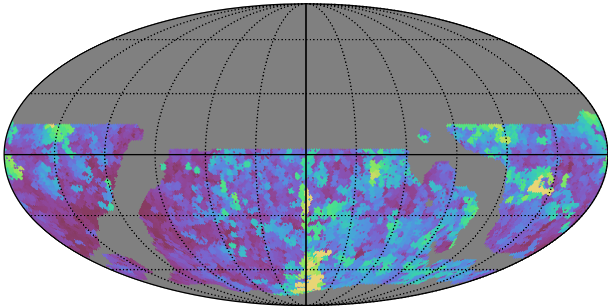
weather_cloudso6v3.4_10yrs WFD z band: Max seeingEff
