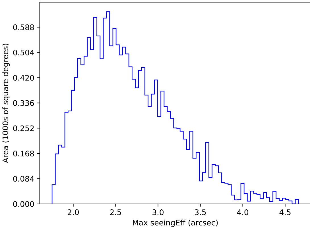
weather_cloudso6v3.4_10yrs WFD z band: Max seeingEff
