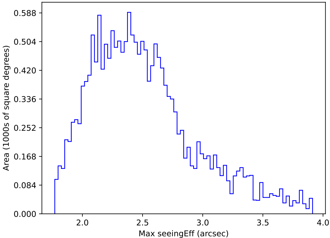
weather_cloudso6v3.4_10yrs WFD u band: Max seeingEff
