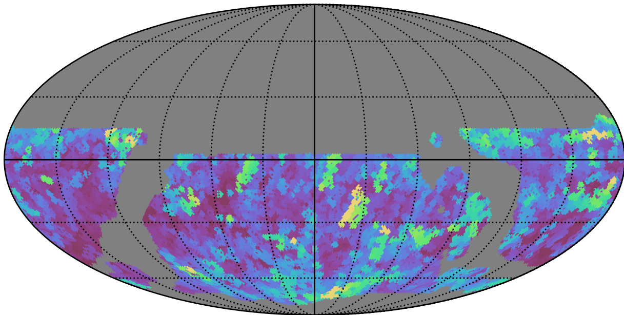
weather_cloudso6v3.4_10yrs WFD r band: Max seeingEff
