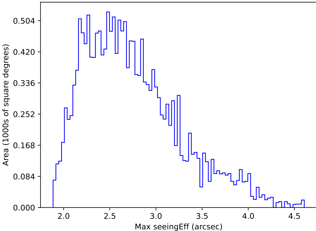
weather_cloudso6v3.4_10yrs WFD r band: Max seeingEff
