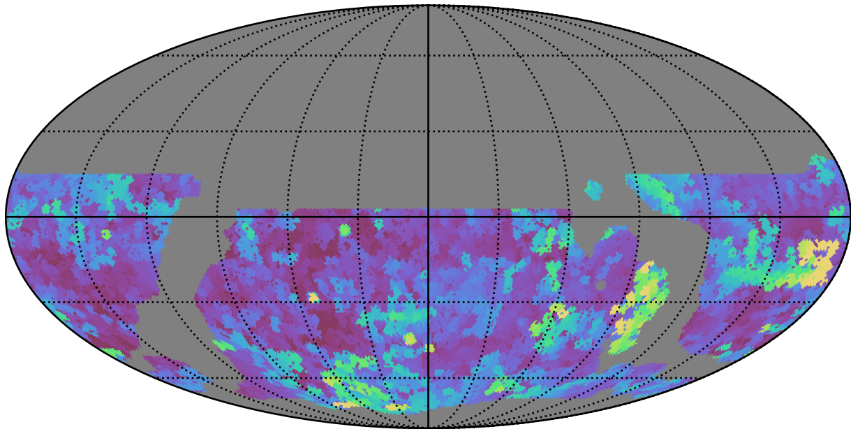
weather_cloudso6v3.4_10yrs WFD g band: Max seeingEff
