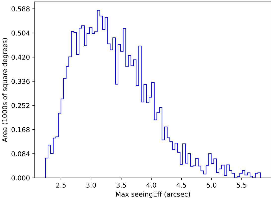
weather_cloudso6v3.4_10yrs WFD all bands: Max seeingEff
