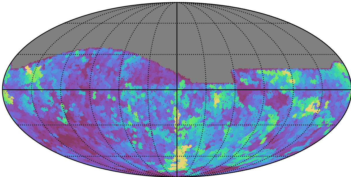
weather_cloudso6v3.4_10yrs All sky z band: Max seeingEff
