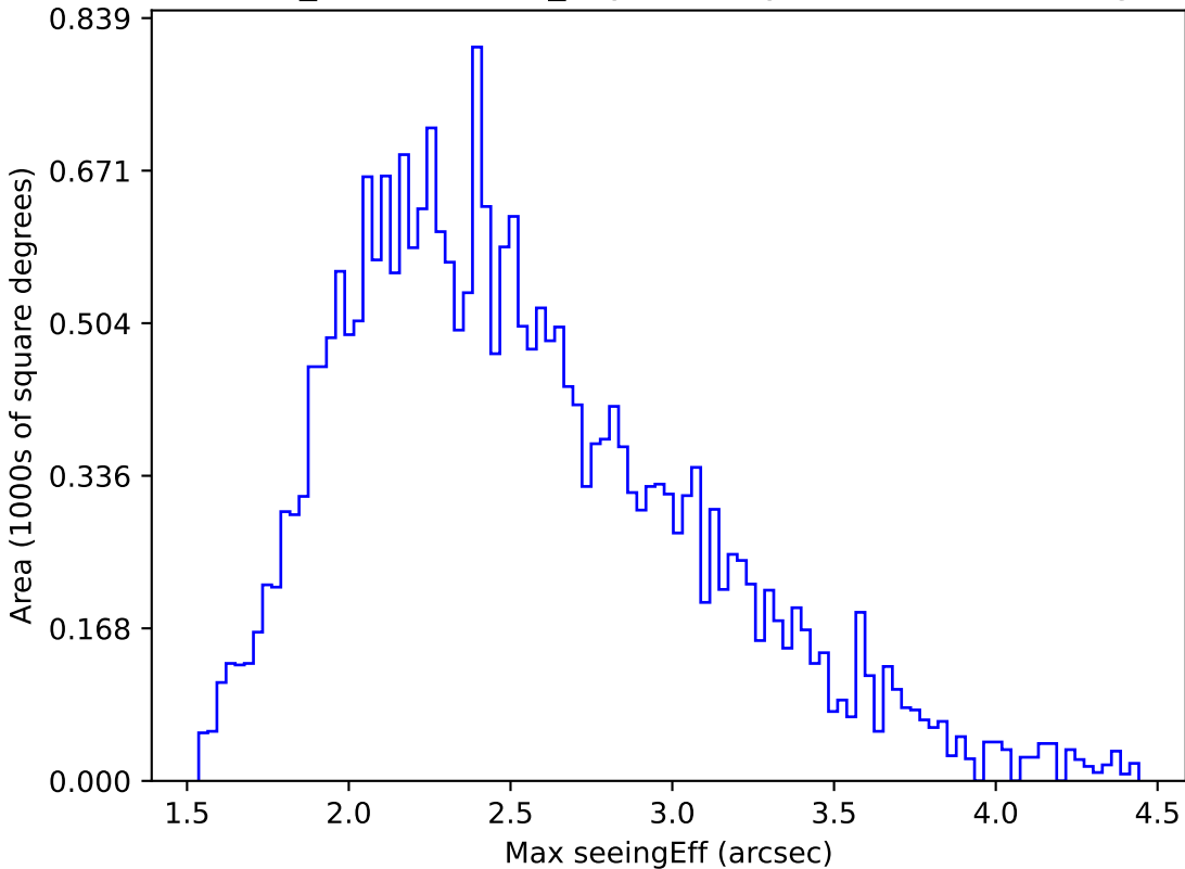
weather_cloudso6v3.4_10yrs All sky z band: Max seeingEff
