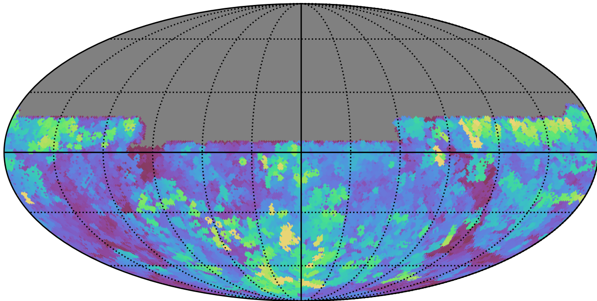
weather_cloudso6v3.4_10yrs All sky u band: Max seeingEff
