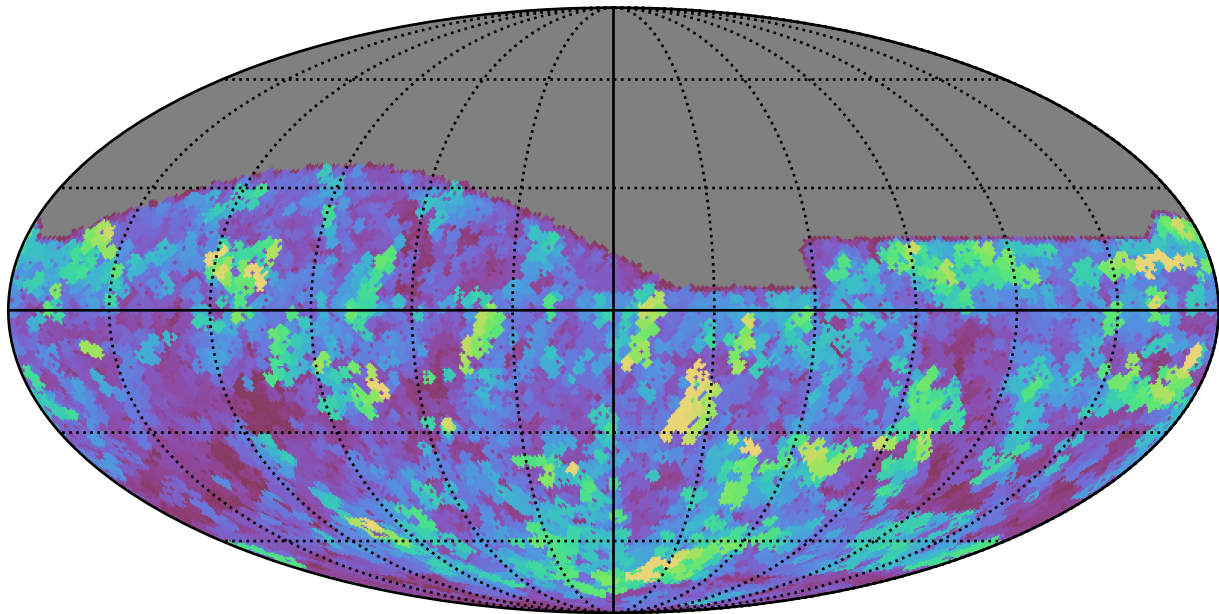
weather_cloudso6v3.4_10yrs All sky r band: Max seeingEff
