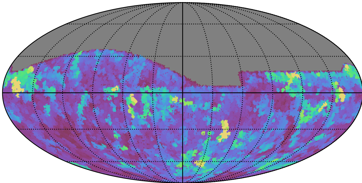
weather_cloudso6v3.4_10yrs All sky i band: Max seeingEff
