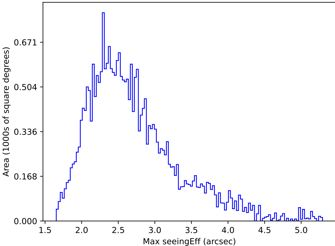
weather_cloudso6v3.4_10yrs All sky i band: Max seeingEff
