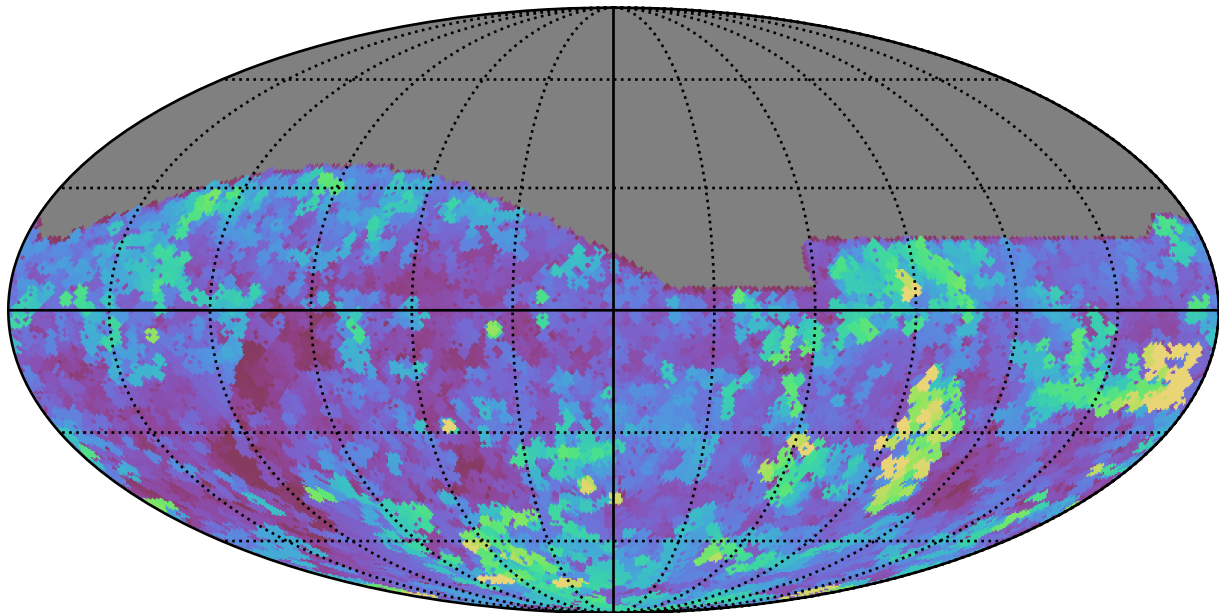
weather_cloudso6v3.4_10yrs All sky g band: Max seeingEff
