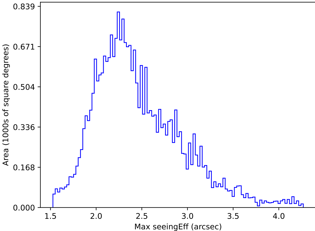
weather_cloudso6v3.4_10yrs All sky g band: Max seeingEff
