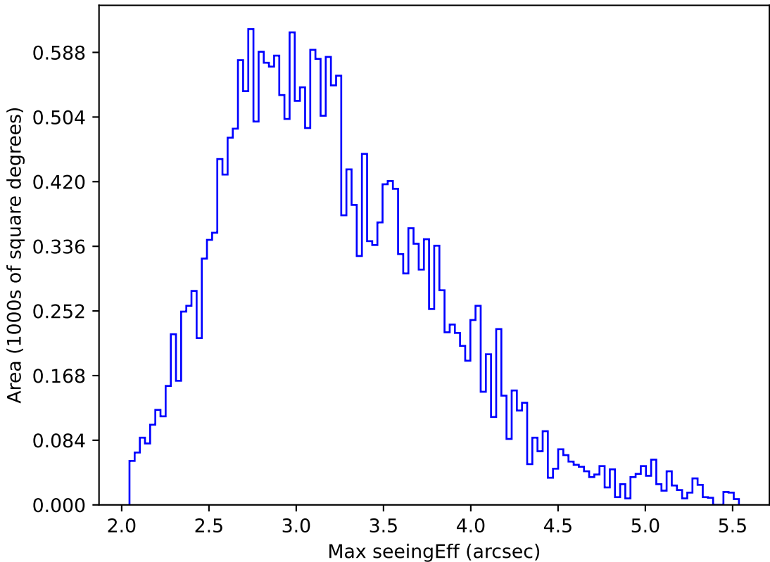
weather_cloudso6v3.4_10yrs All sky all bands: Max seeingEff
