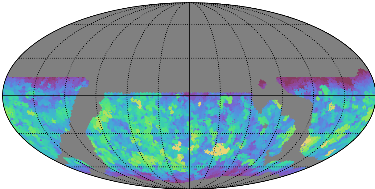
weather_cloudso6v3.4_10yrs WFD all bands: Max saturation_mag
