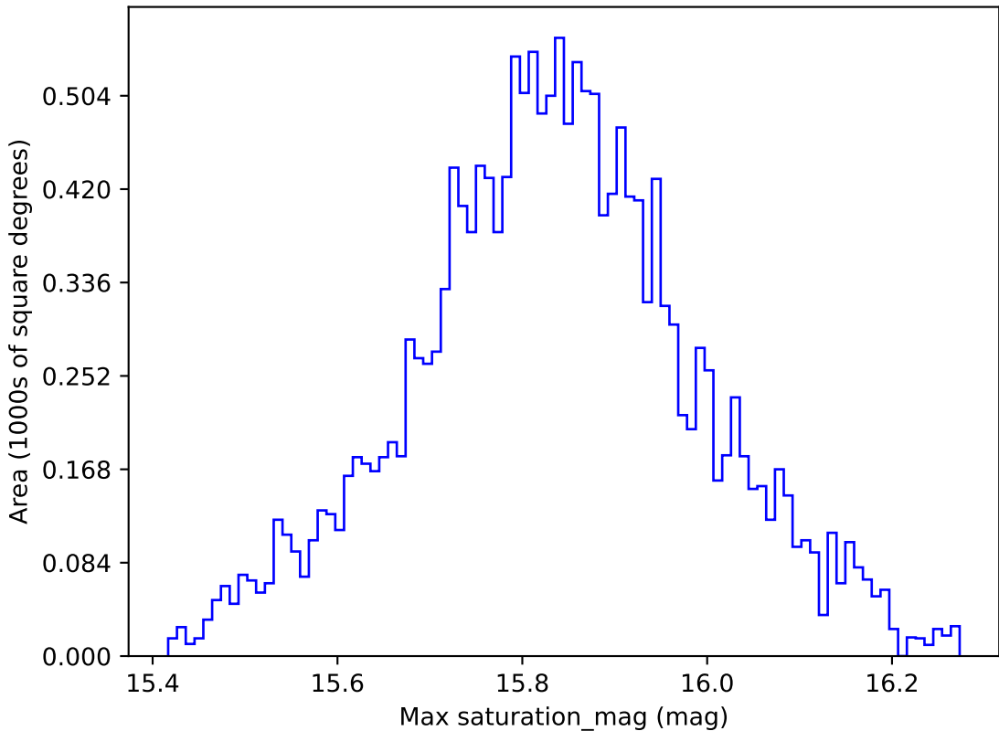
weather_cloudso6v3.4_10yrs WFD all bands: Max saturation_mag
