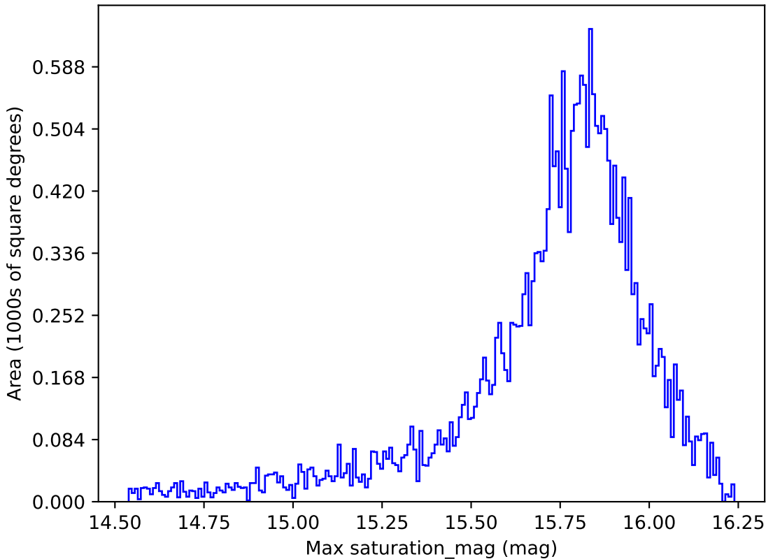
weather_cloudso6v3.4_10yrs All sky all bands: Max saturation_mag
