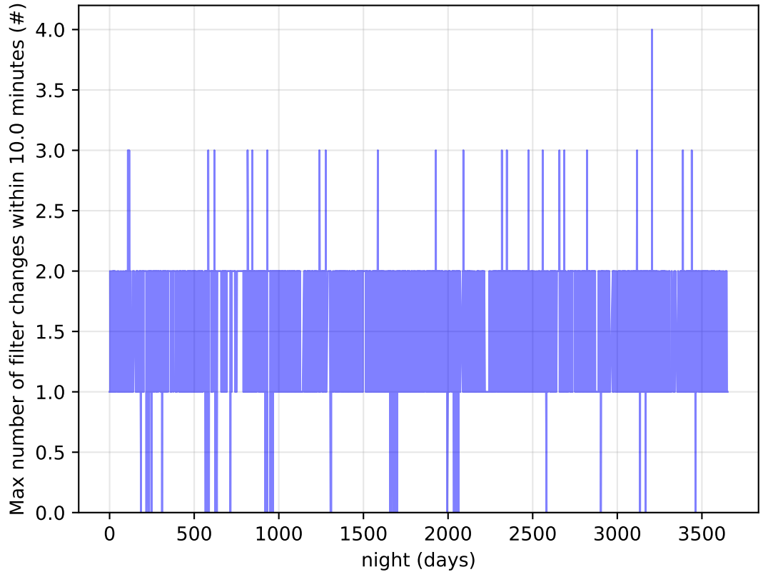
weather_cloudso6v3.4_10yrs Per Night: Max number of filter changes within 10.0 minutes
