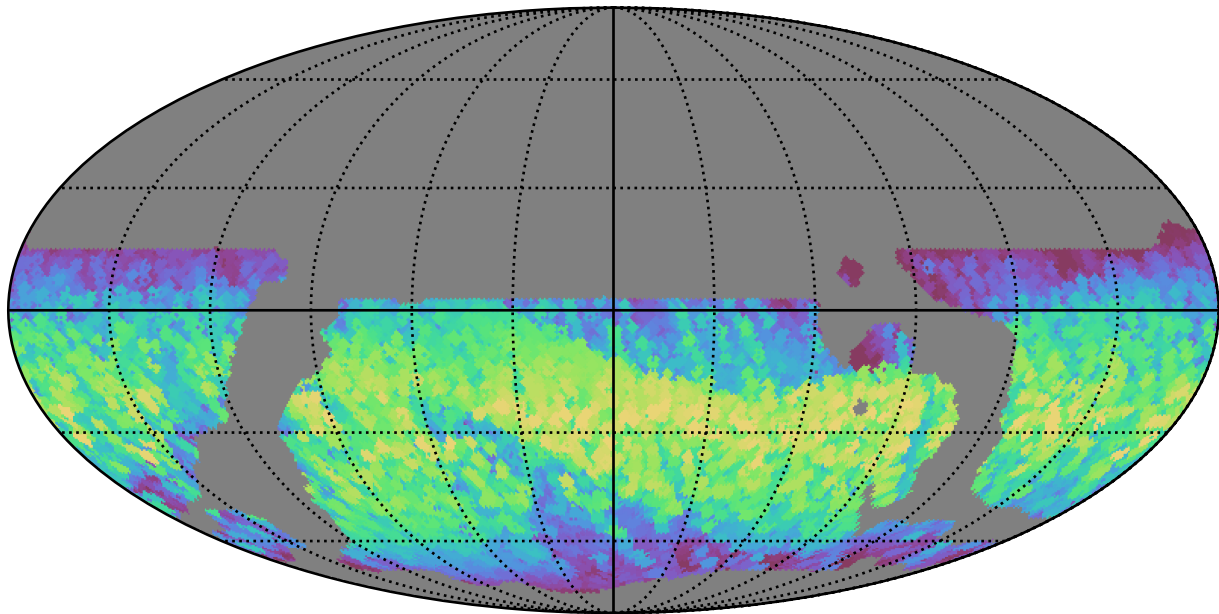
weather_cloudso6v3.4_10yrs WFD all bands: Max normairmass
