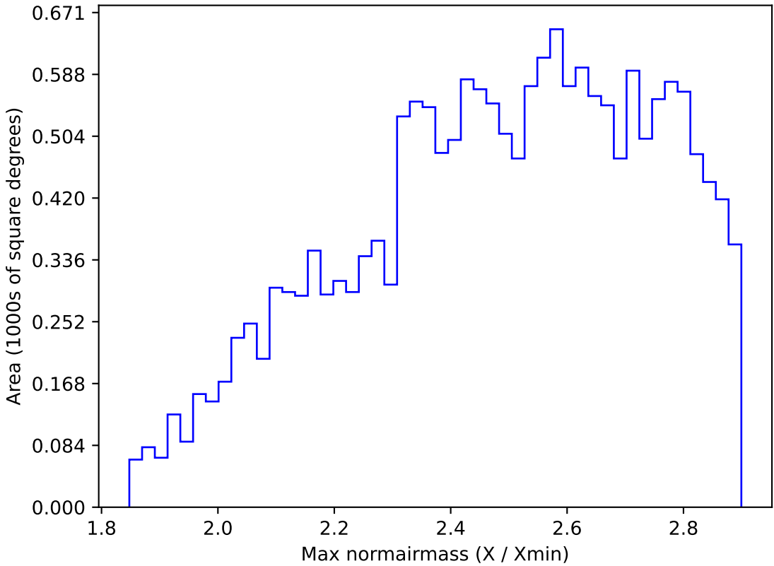
weather_cloudso6v3.4_10yrs WFD all bands: Max normairmass
