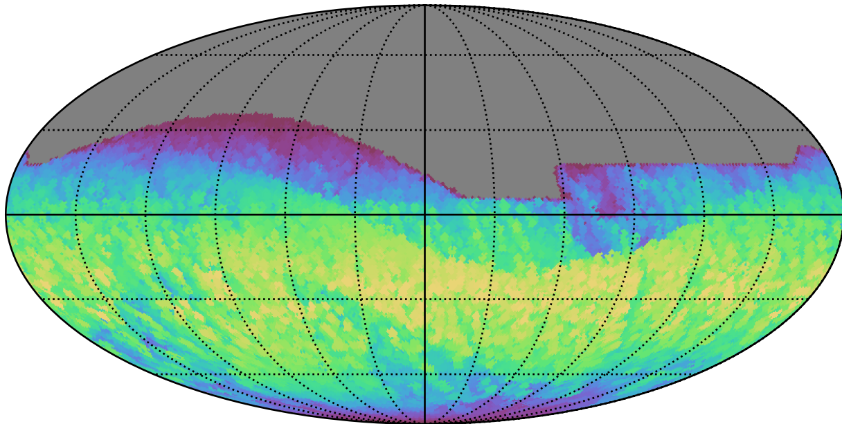
weather_cloudso6v3.4_10yrs All sky all bands: Max normairmass
