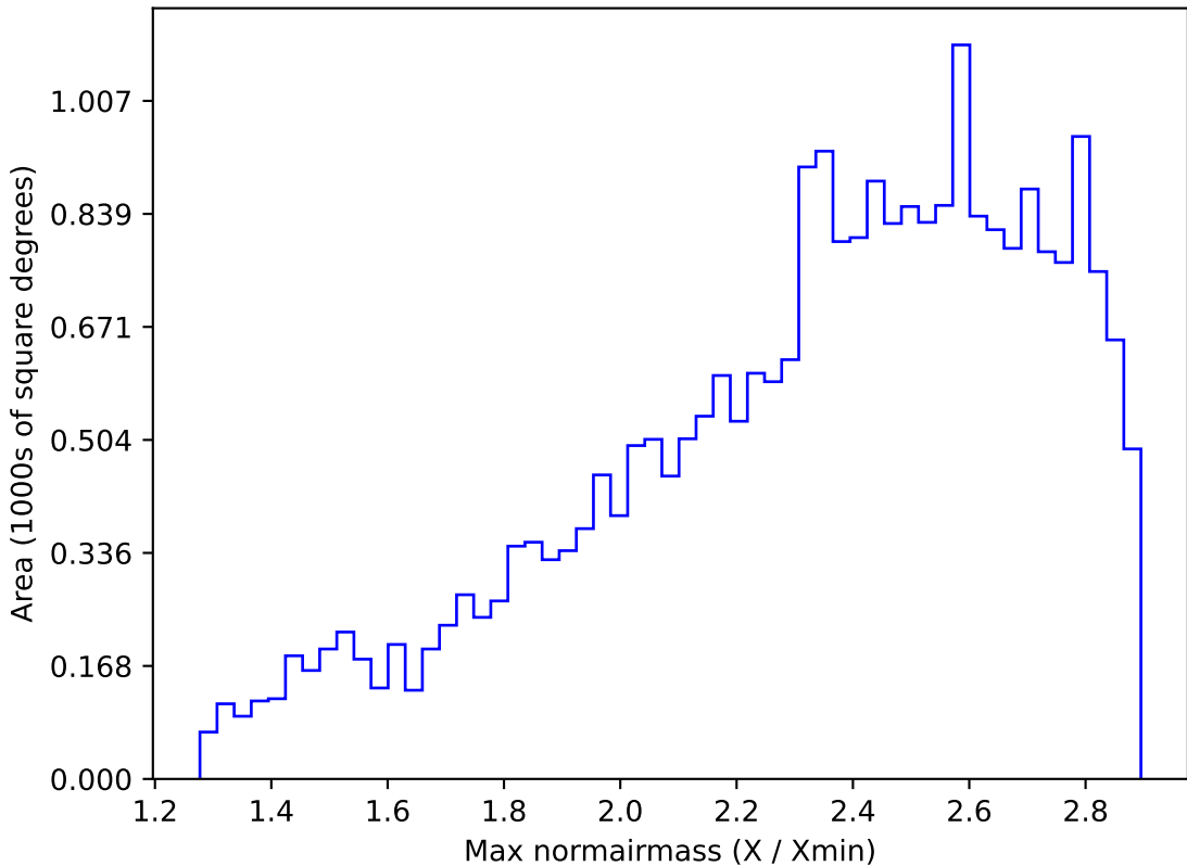
weather_cloudso6v3.4_10yrs All sky all bands: Max normairmass
