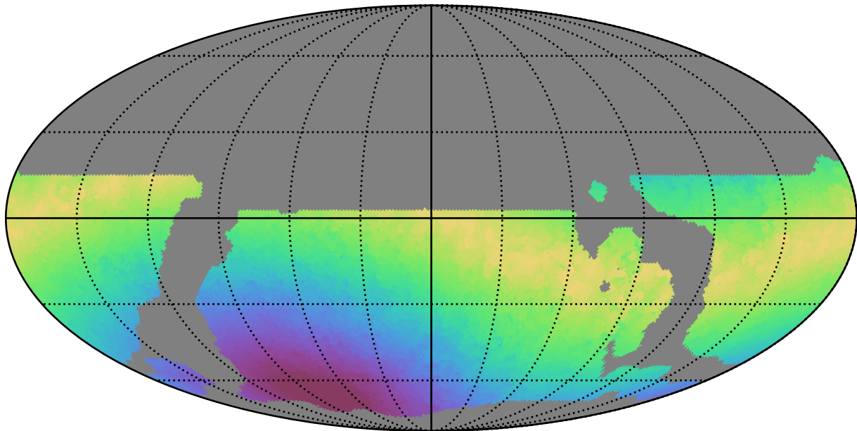
weather_cloudso6v3.4_10yrs WFD z band: Max moonDistance
