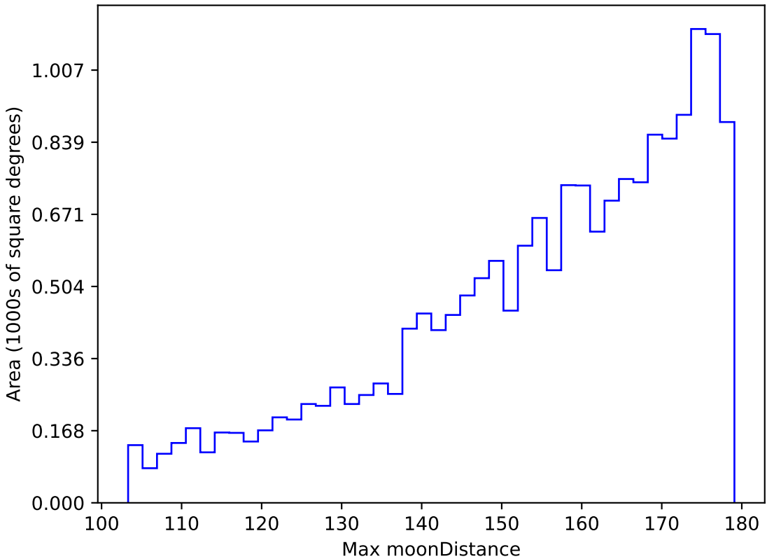
weather_cloudso6v3.4_10yrs WFD z band: Max moonDistance
