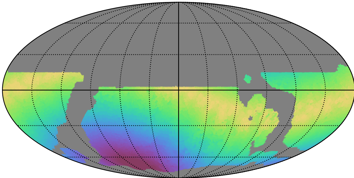
weather_cloudso6v3.4_10yrs WFD u band: Max moonDistance
