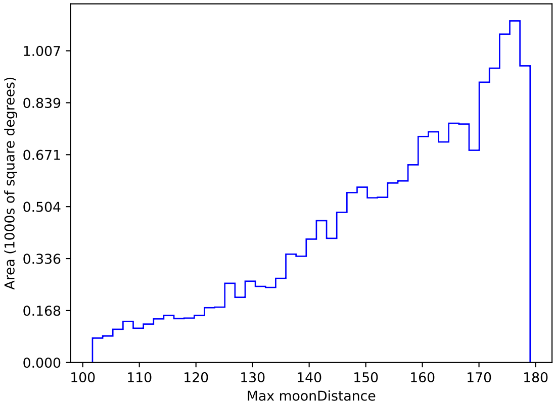
weather_cloudso6v3.4_10yrs WFD u band: Max moonDistance
