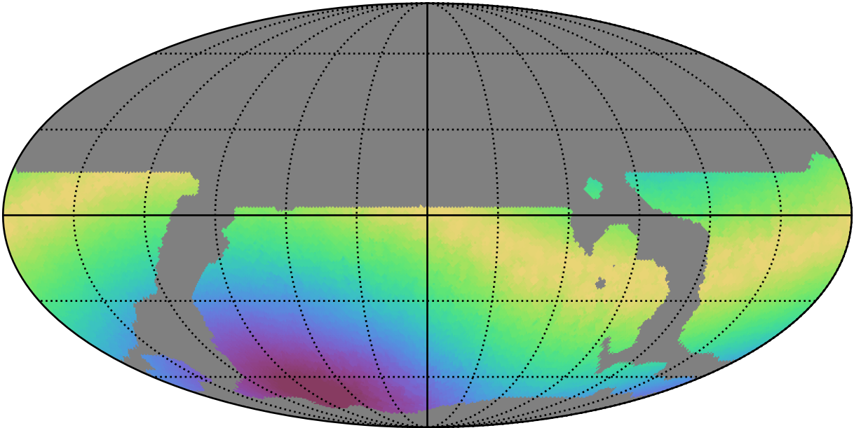
weather_cloudso6v3.4_10yrs WFD r band: Max moonDistance
