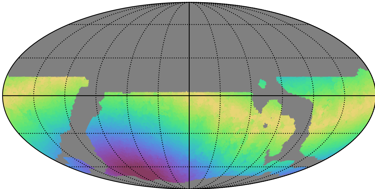
weather_cloudso6v3.4_10yrs WFD g band: Max moonDistance
