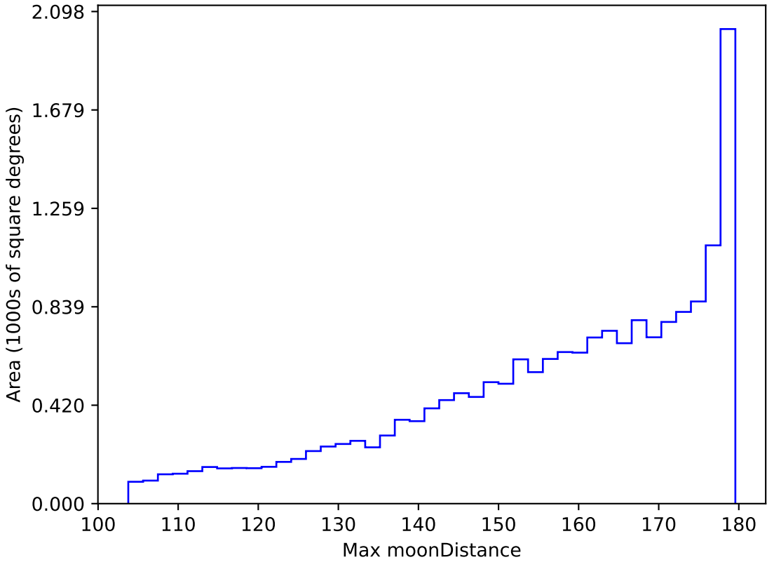
weather_cloudso6v3.4_10yrs WFD all bands: Max moonDistance
