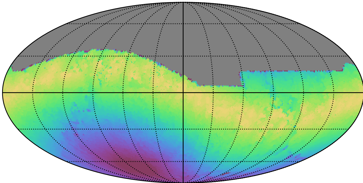
weather_cloudso6v3.4_10yrs All sky z band: Max moonDistance
