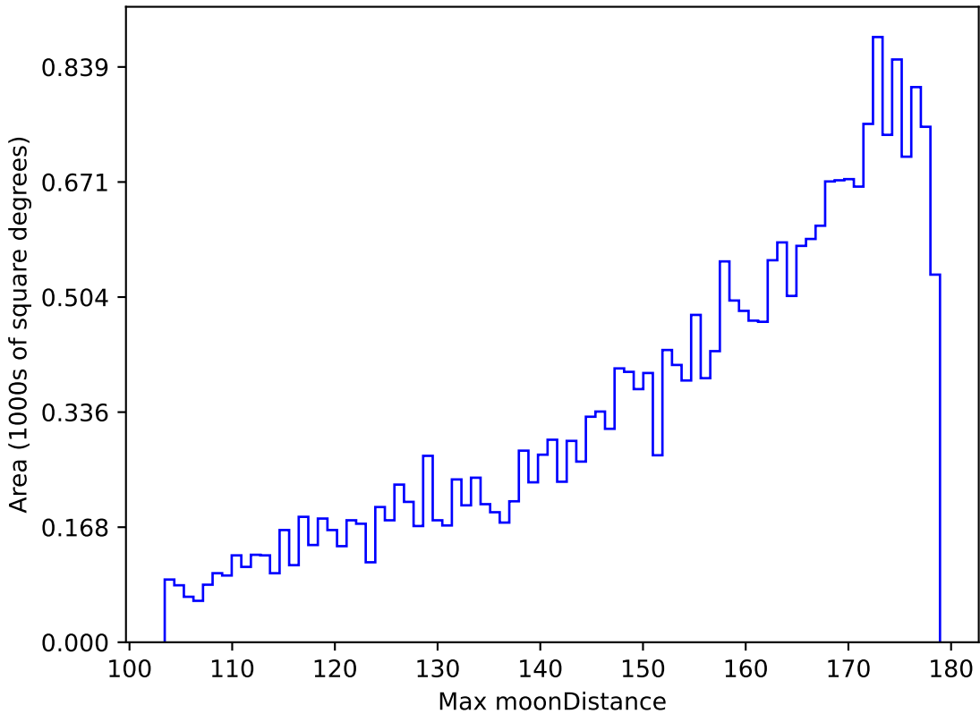
weather_cloudso6v3.4_10yrs All sky z band: Max moonDistance
