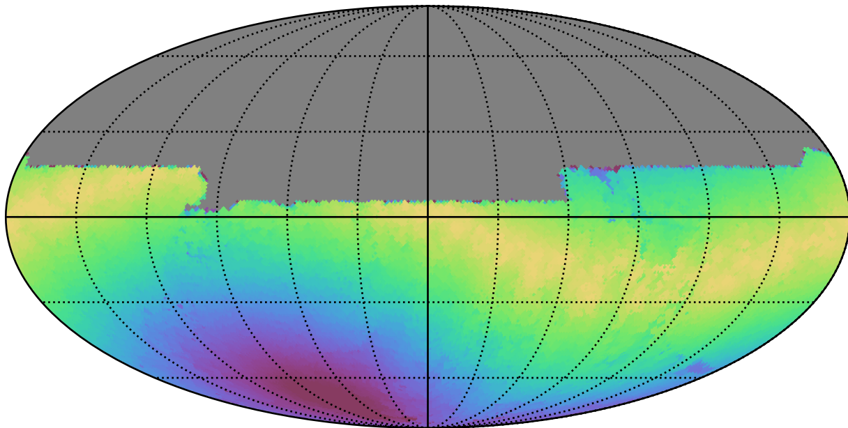
weather_cloudso6v3.4_10yrs All sky u band: Max moonDistance
