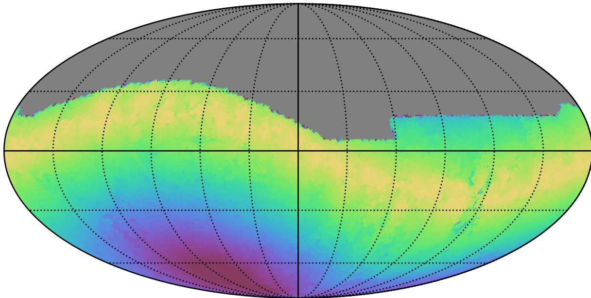
weather_cloudso6v3.4_10yrs All sky g band: Max moonDistance
