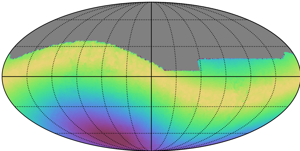
weather_cloudso6v3.4_10yrs All sky all bands: Max moonDistance
