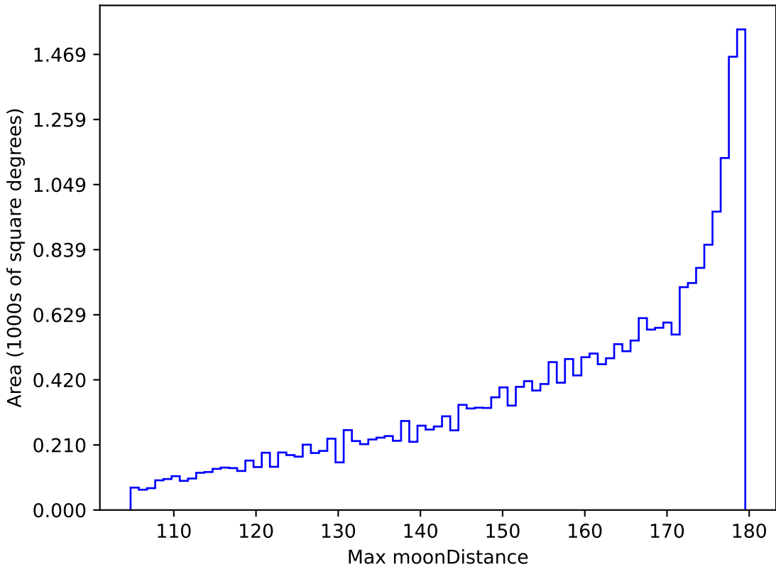
weather_cloudso6v3.4_10yrs All sky all bands: Max moonDistance
