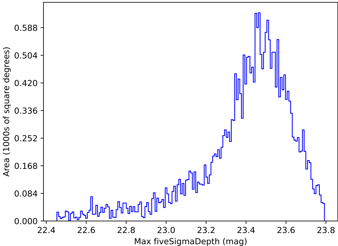
weather_cloudso6v3.4_10yrs Yr 1 z band: Max fiveSigmaDepth
