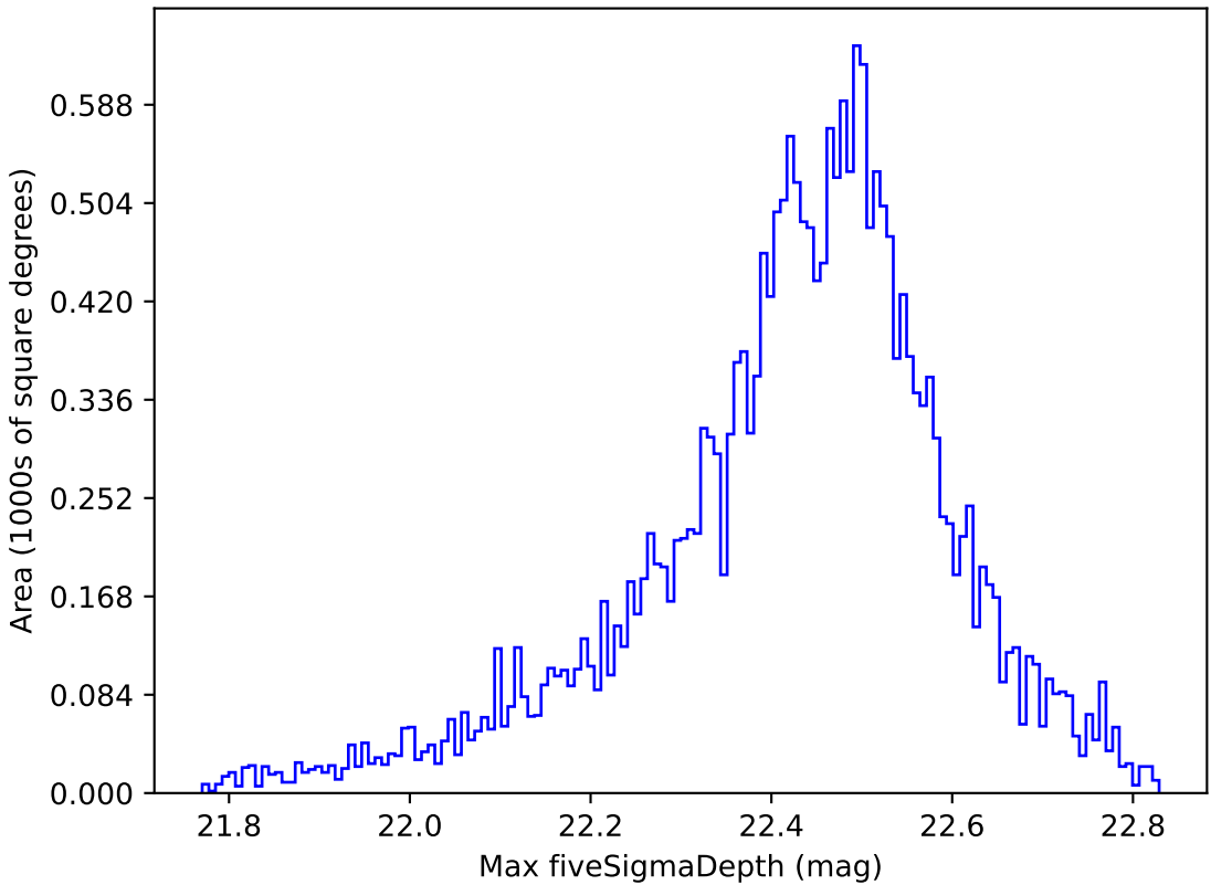
weather_cloudso6v3.4_10yrs Yr 1 y band: Max fiveSigmaDepth
