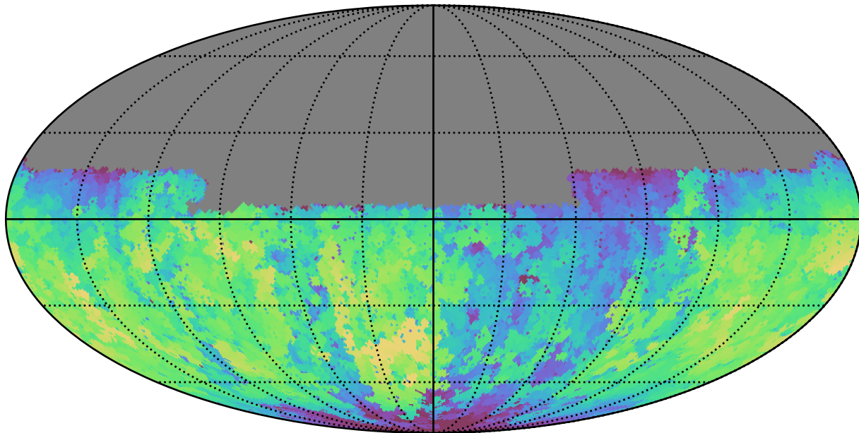
weather_cloudso6v3.4_10yrs Yr1 u band: Max fiveSigmaDepth
