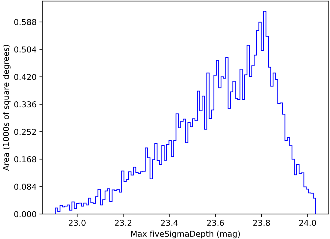
weather_cloudso6v3.4_10yrs Yr 1 u band: Max fiveSigmaDepth
