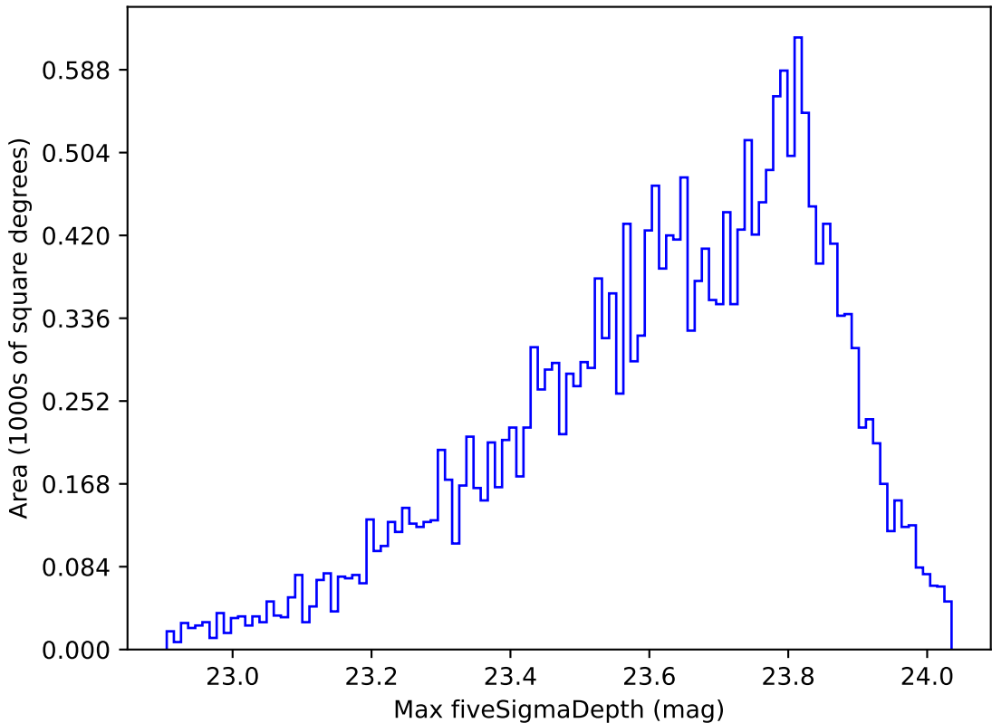
weather_cloudso6v3.4_10yrs Yr 1 u band: Max fiveSigmaDepth
