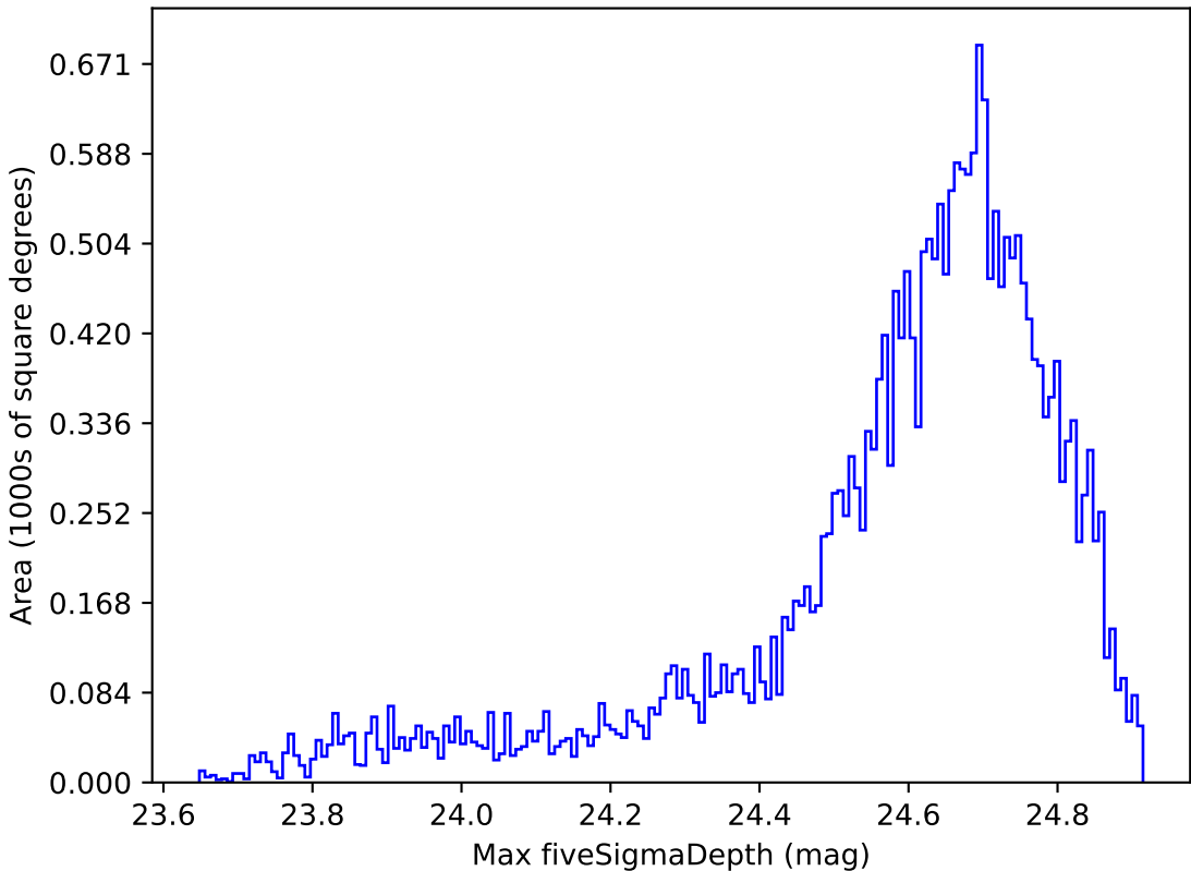
weather_cloudso6v3.4_10yrs Yr 1 r band: Max fiveSigmaDepth
